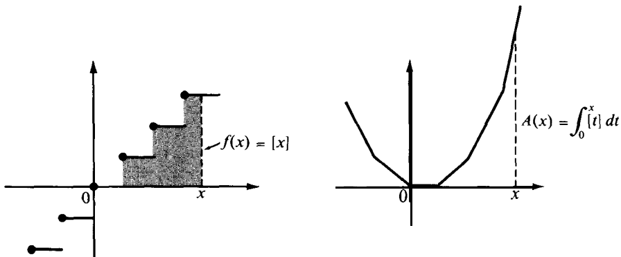
FIGURE 2.17 The indefinite integral of a step function is piecewise linear.
