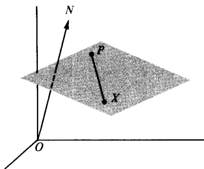
FIGURE 13.7 A plane through \mathbf{P} and X with normal vector \mathbf{N} .
