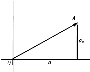
FIGURE 12.7 In V_2 , the length of A is \sqrt{a_1^2 + a_2^2} .
