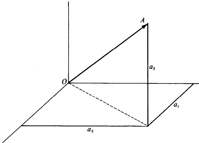
FIGURE 12.8 In V_3 , the length of A is \sqrt{a_1^2 + a_2^2 + a_3^2} .
