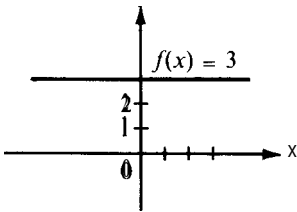
FIGURE 1.8 A constant function f(x) = 3 .
